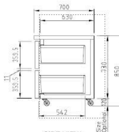
SIDE VIEW (Depth 700mm)
