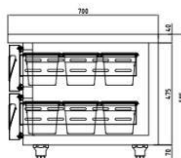
TCB-SERIES SIDE VIEW
